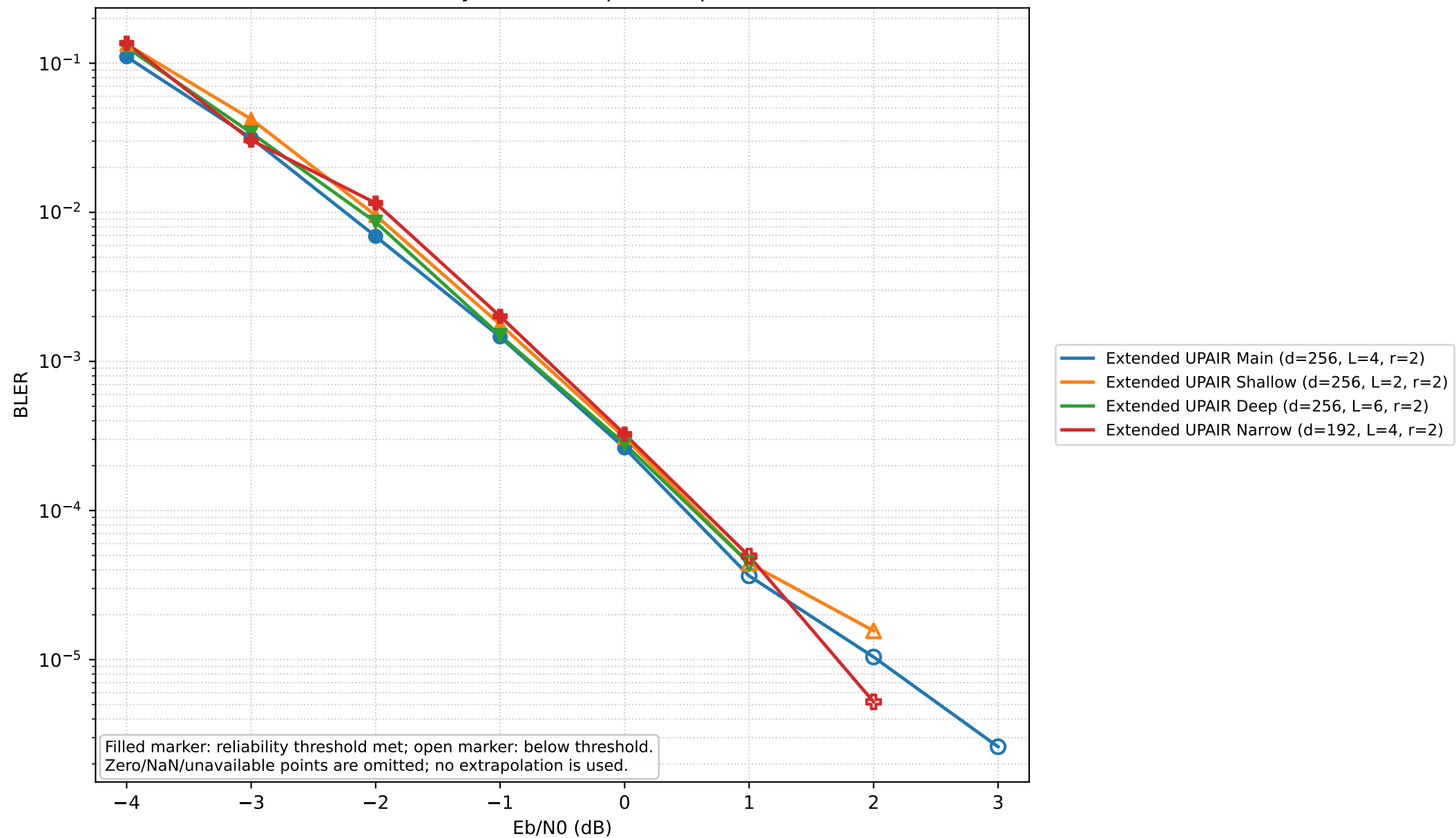
Extended UPAIR Architecture Comparison — BLER 3 active users — only evaluated, positive points are shown
